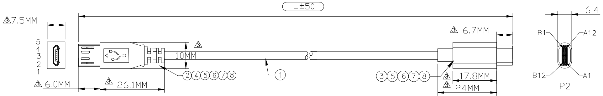
P1 MICRO USB(B)M 5P (MOLDING BLACK COLOR)
